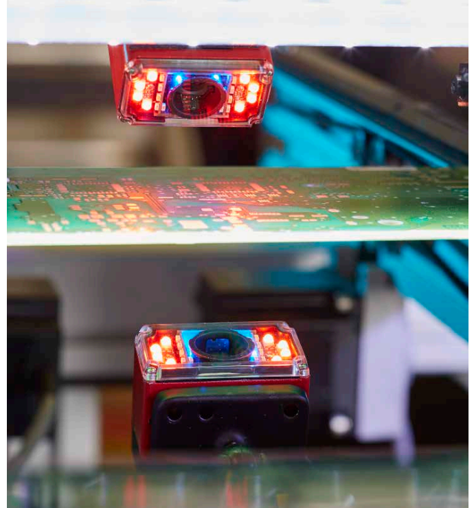
MicroHAWK cameras gather data from miniscule codes placed on a circuit board.
